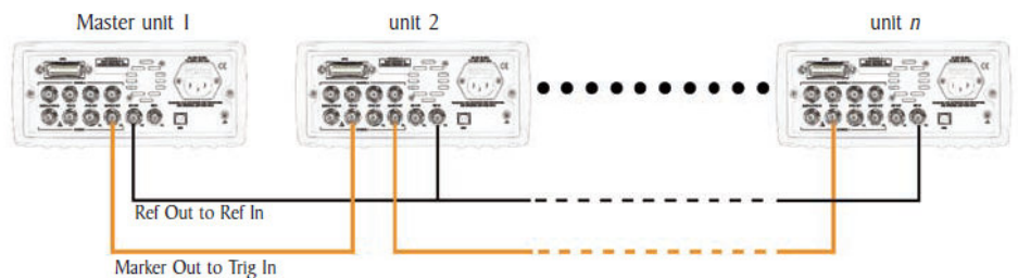
Multi-unit/channel synchronization
